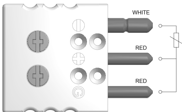
Leadwire Resistance
