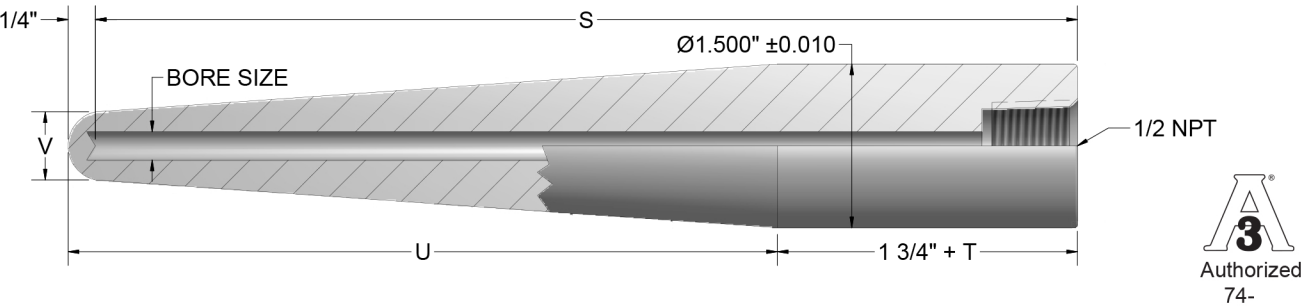
Thermowell Dimensions
